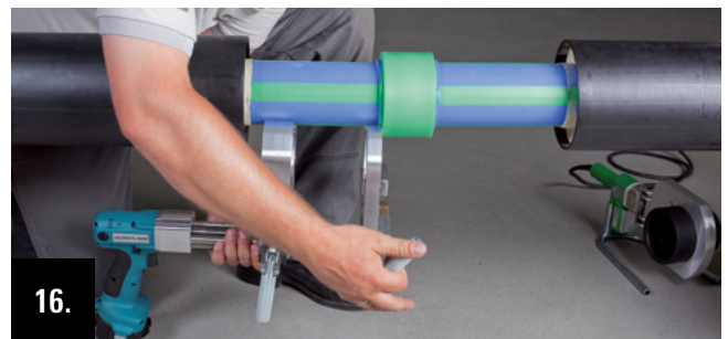
16. Open the clamping jaws of the welding jig as far that the welding jig can be removed sidewise or downward from the connection.
