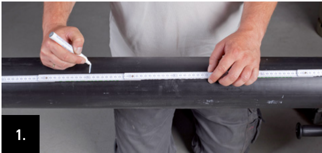
1. Measure the pipe length and mark on the casing pipe.
