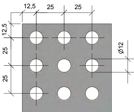
Straight round punching 12/25 R
