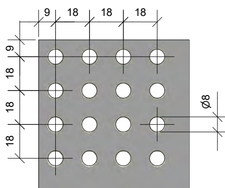
Straight round punching 8/18 R
